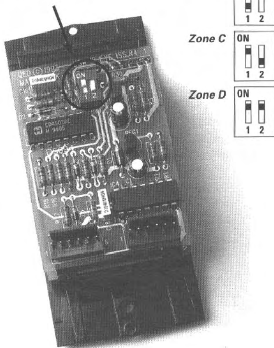
Zone switches
