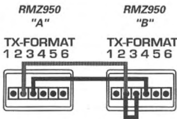
Use this jumper arrangement in a system with 2 RMZ950 controllers to enable the flood IR emitters on both RMZ950 controllers.
